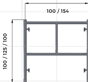
QUADROS "LV"
